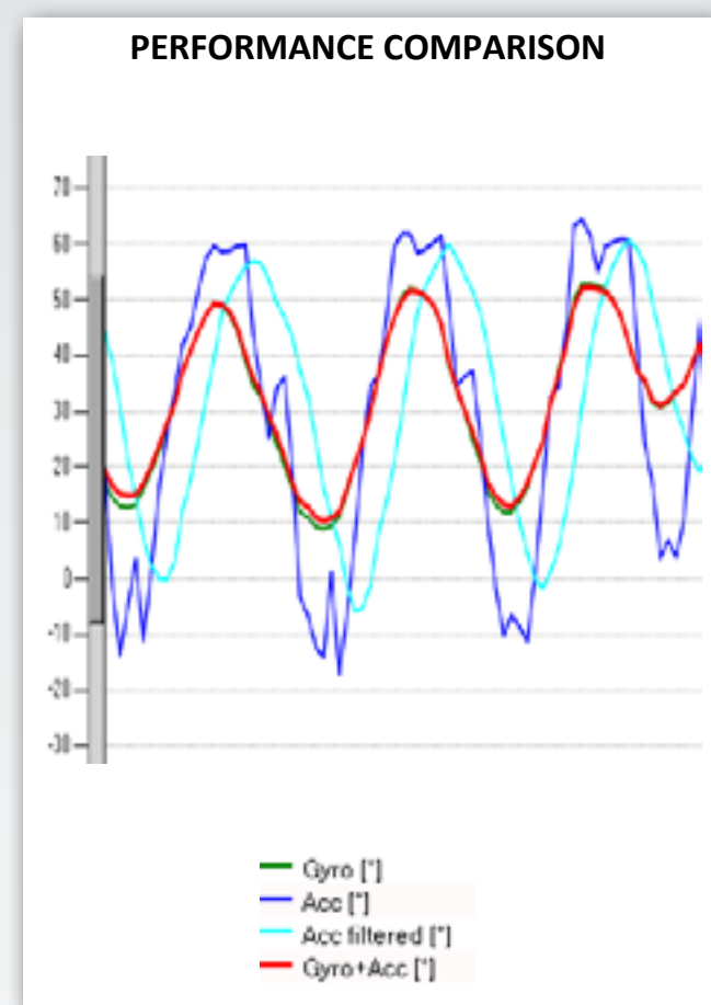
INCLINOMETER WITH INTEGRATED GYROSCOPE
